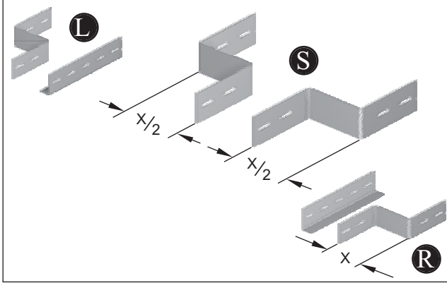
Z Reduction plates
