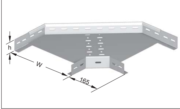
Rigid bend 90° perforated Heavy duty design Small bend 90° R= 165 mm.
