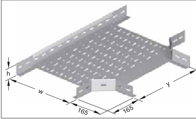
Tee perforated Heavy duty design
