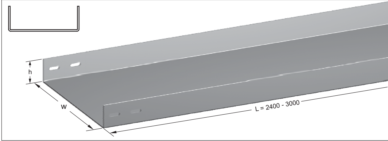
Cable Tray unperforated (Standart design.)
