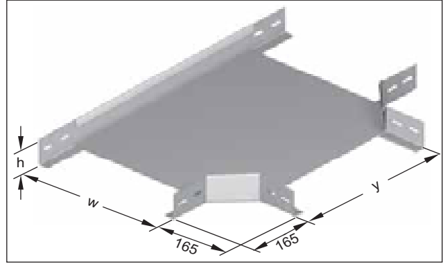
Tee unperforated Heavy duty design
