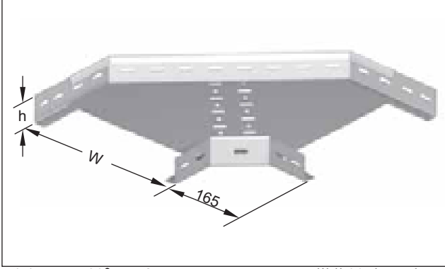
Rigid bend 90° perforated Heavy duty design
