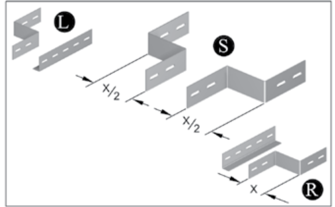
Z Reduction plates
