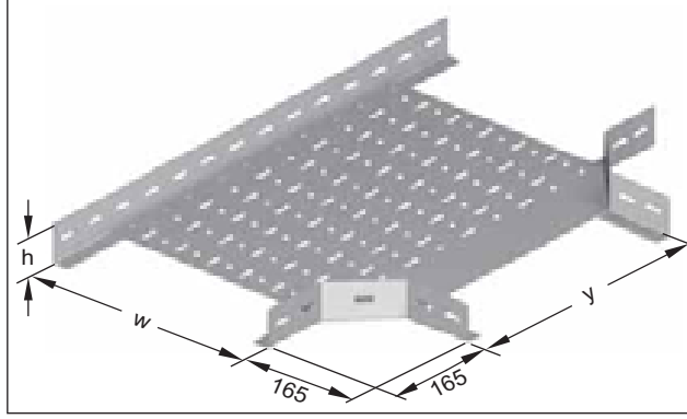
Tee perforated Standart type
