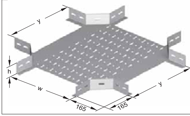
Crossing perforated Standart design
