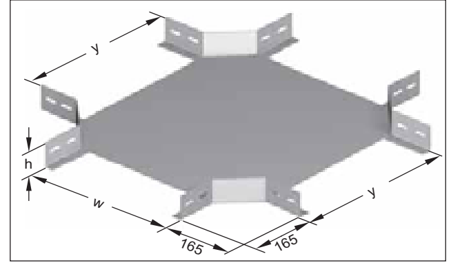
Crossing unperforated Standart design
