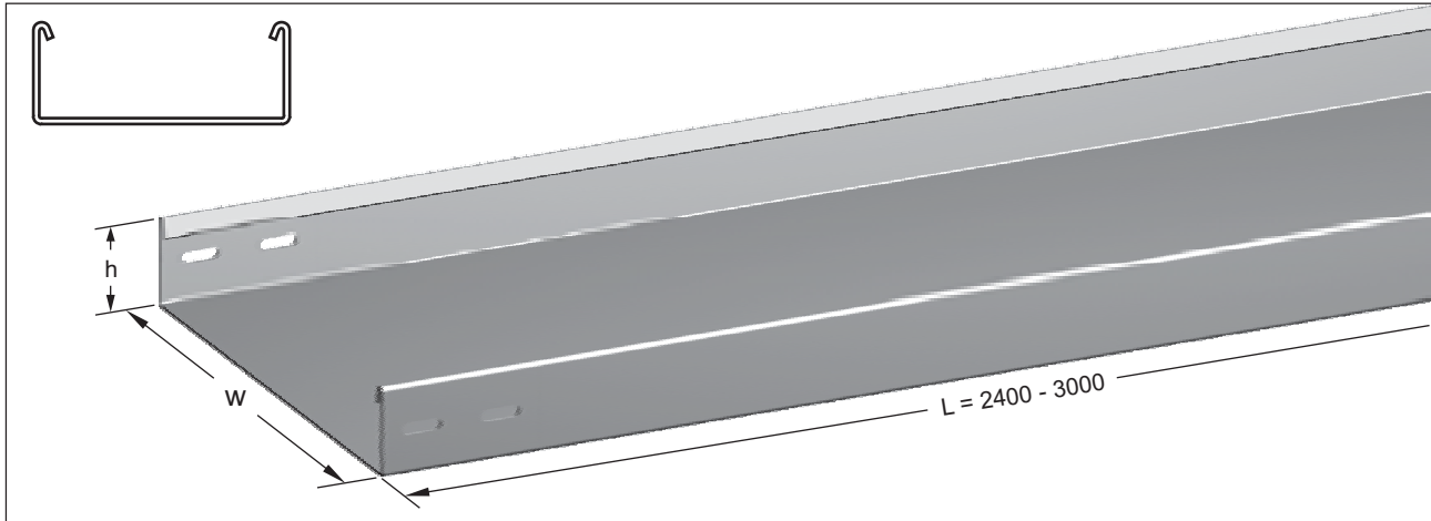
Cable tray unperforated (Heavy duty design.)
