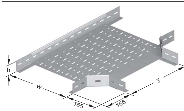
Tee perforated Heavy duty design Small Tee R= 165 mm.
