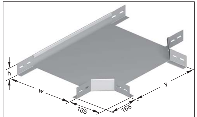
Tee unperforated Heavy duty design Small Tee R= 165 mm.
