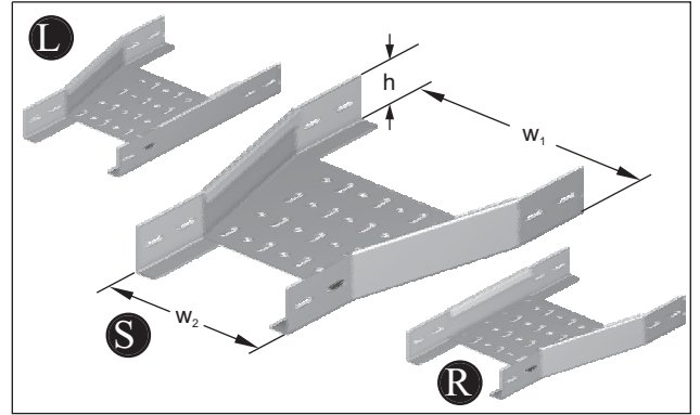
Reduction perforated Heavy duty design
