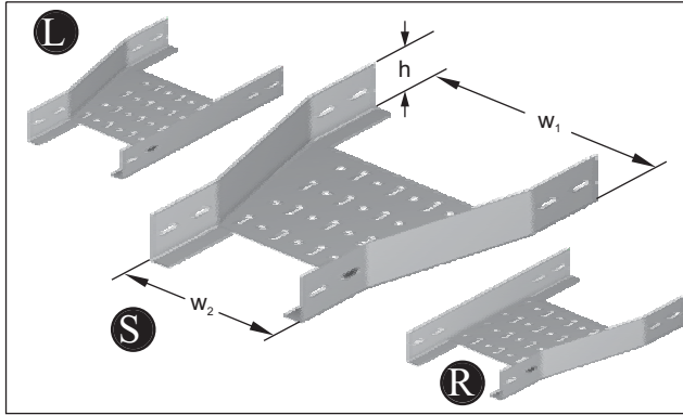
Reduction perforated Standart type
