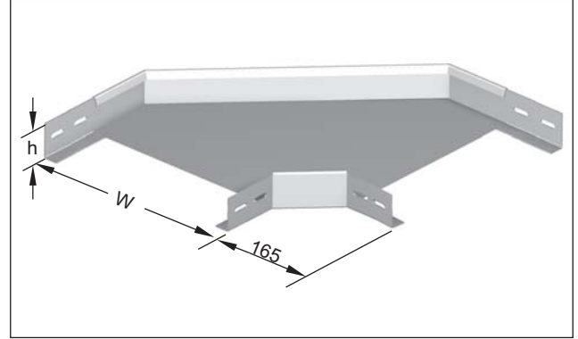
Rigid bend 90° unperforated Heavy duty design Small bend 90° R= 165 mm.
