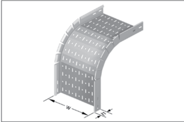
Flexible vertical bend Heavy duty design Perforated
