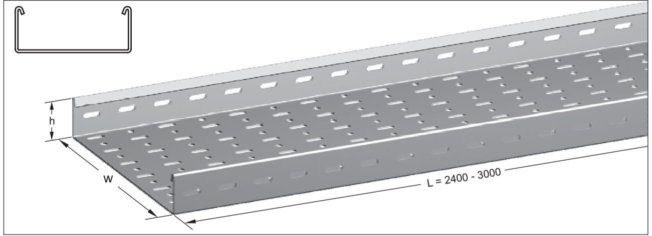
Cable tray perforated (Heavy duty design.)
