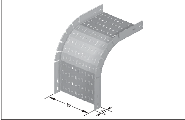
Flexible vertical bend Standart type Perforated
