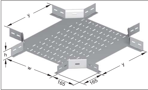
Crossing perforated Heavy duty design Small Crossing R= 165 mm.
