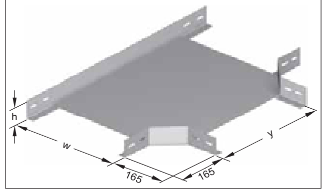
Tee unperforated Standart type
