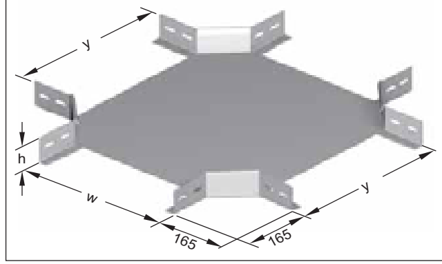
Crossing unperforated Heavy duty design Small Crossing R= 165 mm.
