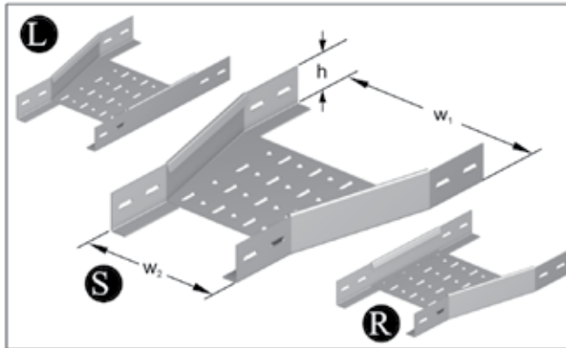
Reduction perforated Heavy duty design
